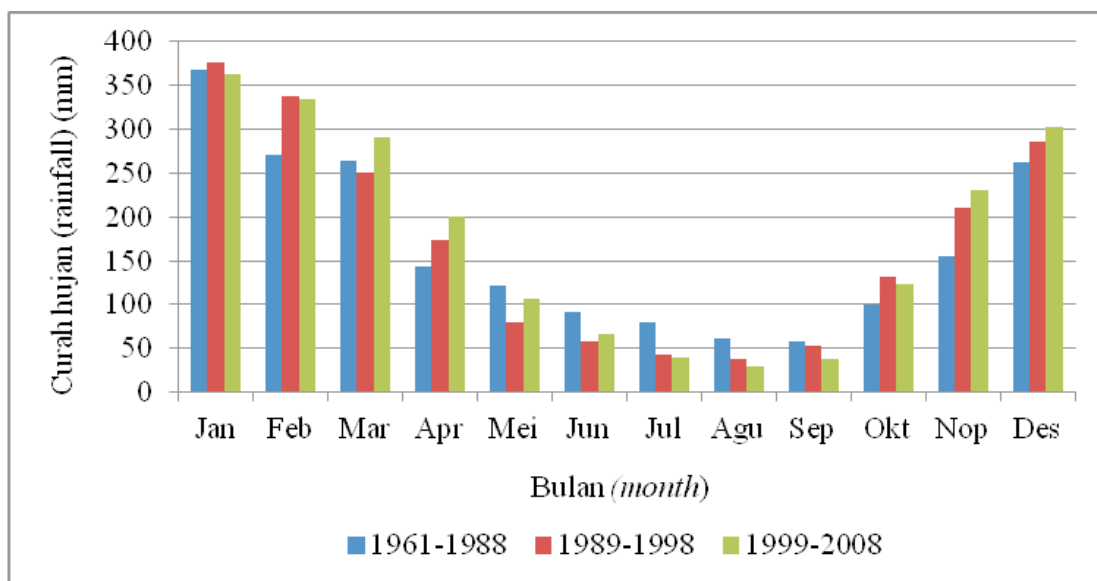
Gambar 3. Curah hujan rata-rata bulanan di pulau Bali Figure 3. Average monthly rainfall in Bali island
