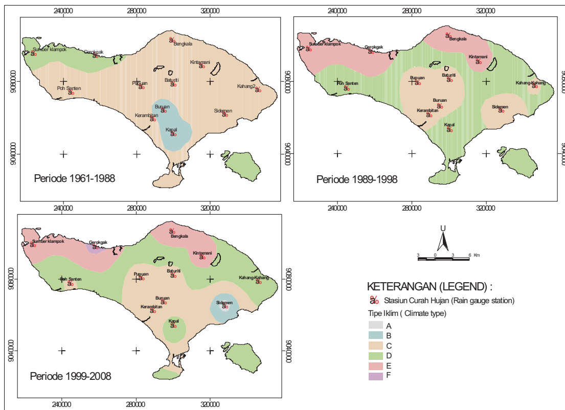
Gambar 6. Penyebaran type iklim di Bali untuk tiap periode Figure 6. Spasial distribution of climate type in Bali for each period
