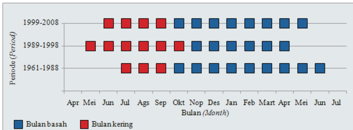
Gambar 7. Perbandingan bulan basah dan kering tiga periode di pulau Bali Figure 7. Comparison of wet and dry month of three periods in Bali island
