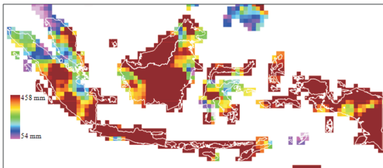
Gambar 1. Ilustrasi distribusi curah hujan dari GPCC format grid di Indonesia Figure 1. Illustration of GPCC grid format rainfall distribution in Indonesia
