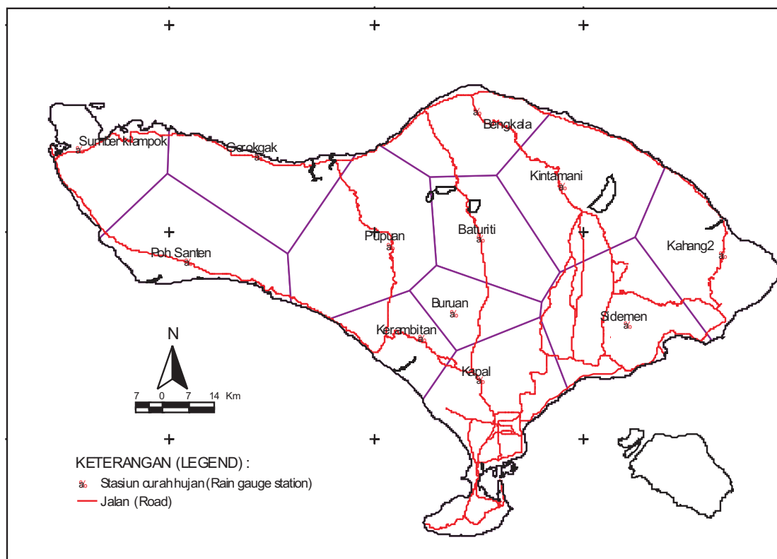
Gambar 2. Peta poligon Thiessen di pulau Bali Figure 2. Thiessen polygon map of Bali island
